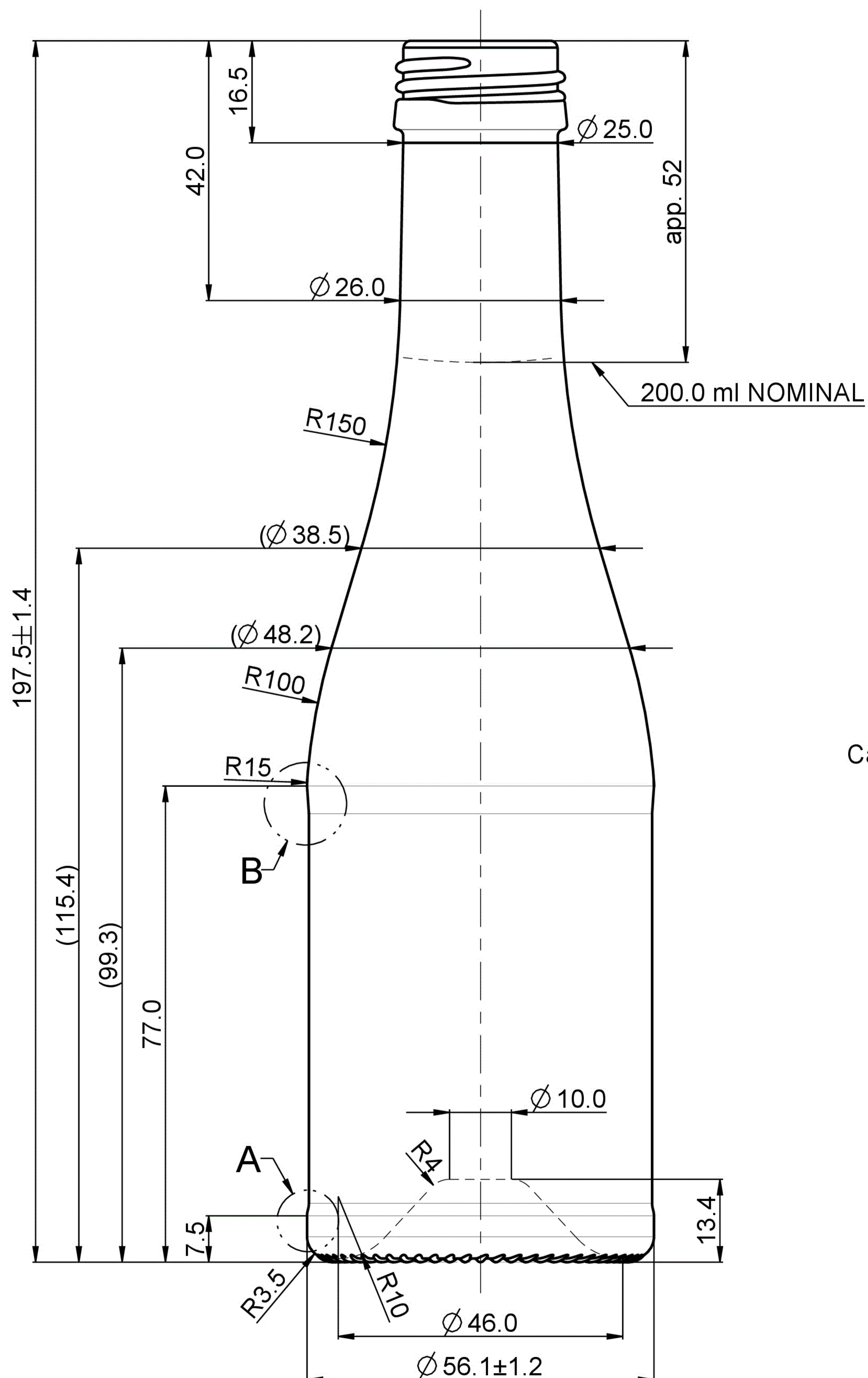
Front view MCA 1 CE.T.I.E. GME 32.00:2008-06
